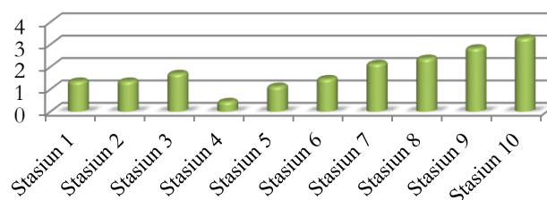
Gambar 5. Persentase Tutupan Lamun
