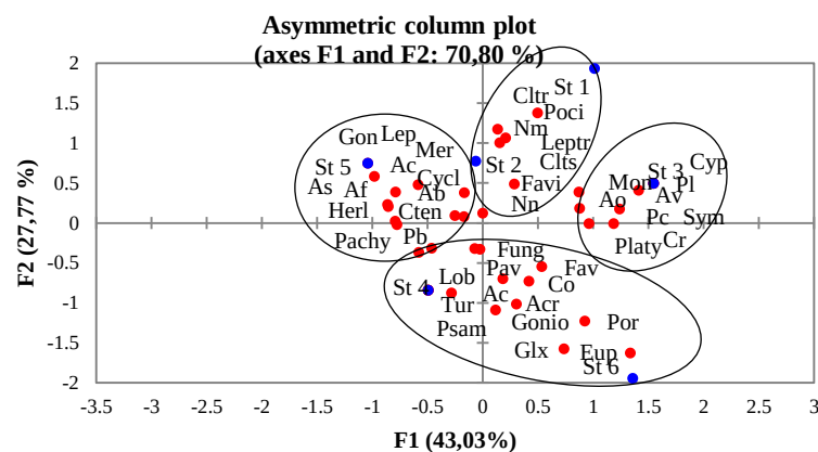
Gambar 4. Diagram hasil analisis koresponden
