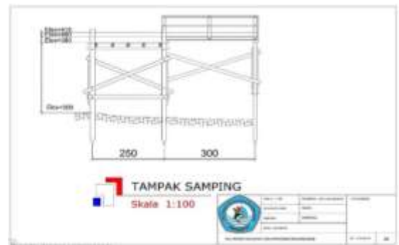
Gambar 7. Desain tampak samping dermaga kano (canoe docks).
