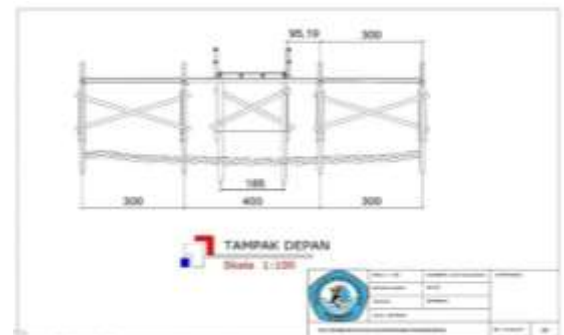
Gambar 8. Desain tampak depan dermaga kano (canoe docks)
