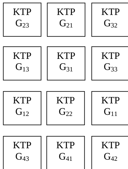
Figure 1. Completely randomized design from each treatment and three replicates affected by Ketapang leaf dose against decreasing content of the heavy metal copper.
