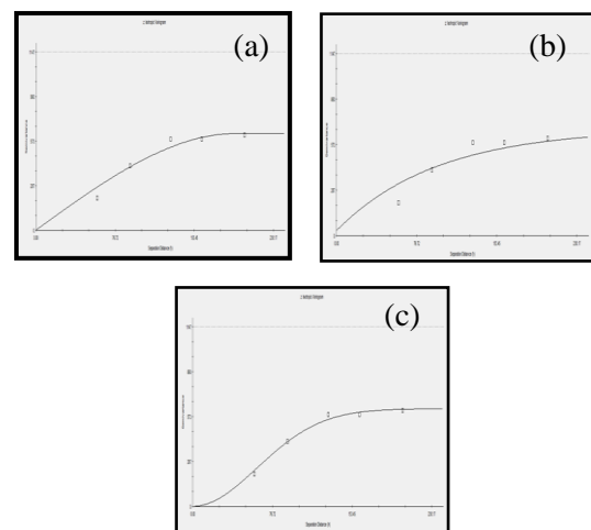
Gambar 5. Model Semivariogram, (a) spherikal; (b) Eksponensial; (c) Gaussian
