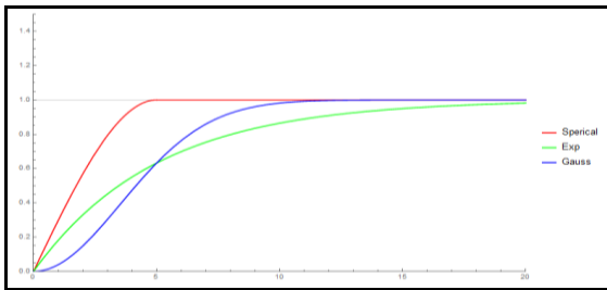
Gambar 1. Model Semivariogram (sferikal, eksponensial dan Gaussian)
