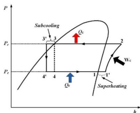
Gambar 3 Diagram P – h
