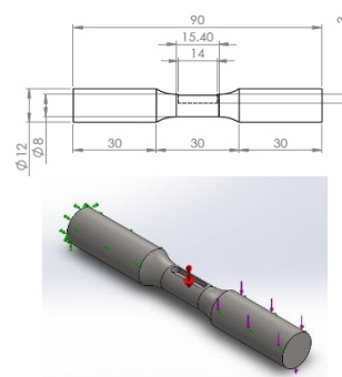
Gambar 1 Standar ASTM E466
