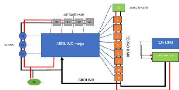
Gambar 1. Diagram Blok
