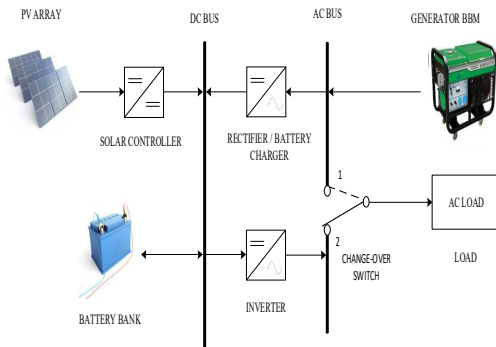
Gambar 2 Sistem Hibrid Switched
