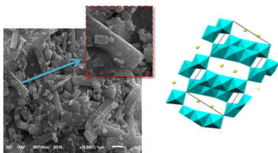
Gambar 2. Arah pertumbuhan \text{Na}_2\text{Ti}_6\text{O}_{13}
